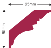
C0019 SMALL ACANTHUS LEAF Length 3000mm Pattern repeat 280mm Part of a co-ordinated collection
