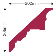
C0052 LEAF DENTIL WITH EGG AND DART Length 2880mm Pattern repeat 80mm
