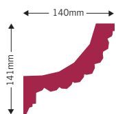
LT 2 REEDED LIGHTING TROUGH Length 1832mm
