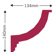
LT 1 PLAIN LIGHTING TROUGH Length 1784mm
