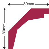
C0100 PLAIN RUN COVE Length 3000mm If desired profile can be inverted
